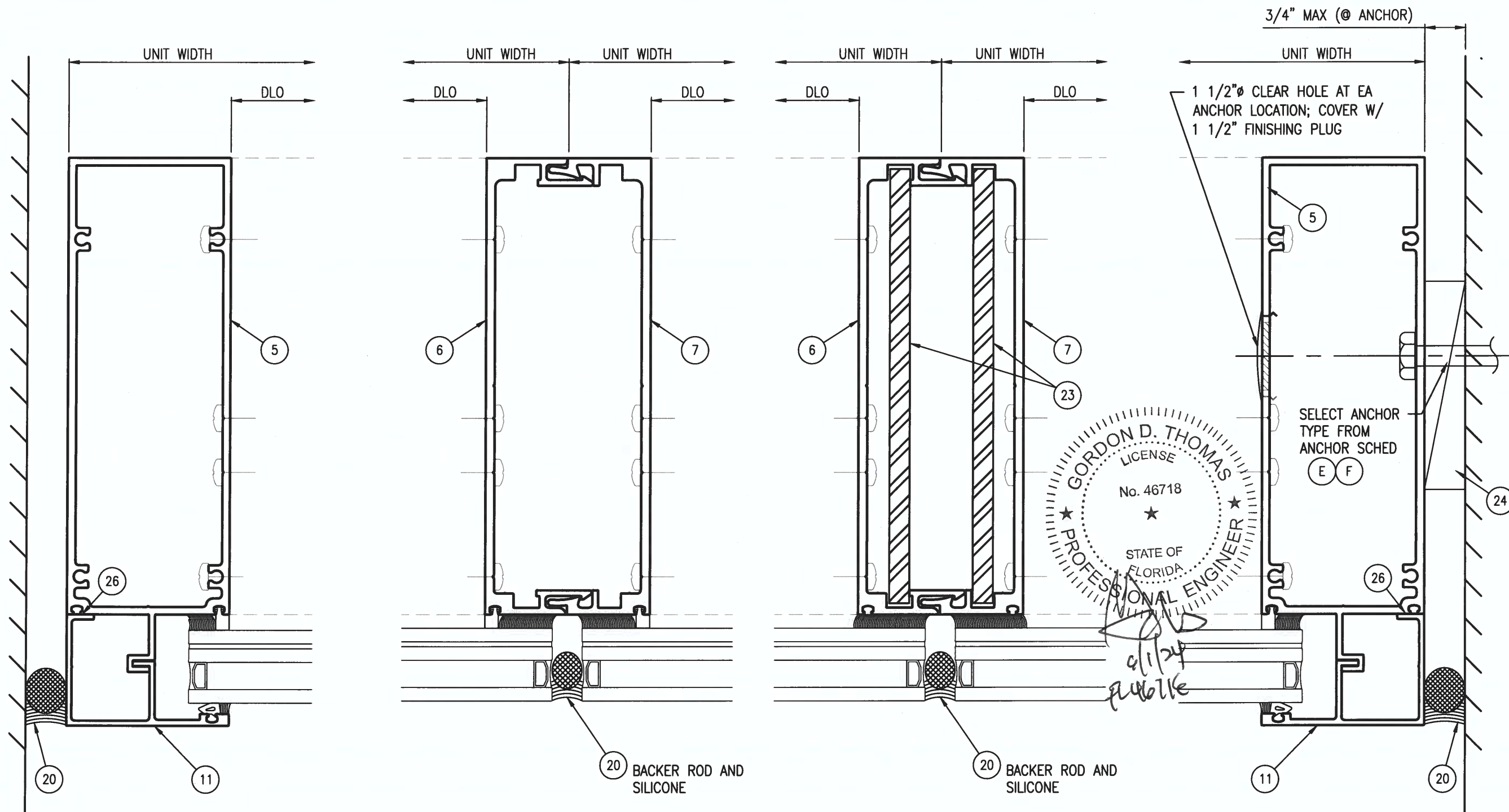
1 UNANCHORED JAMB Glazing condition G2 Scale: 6" = 1'-0"
